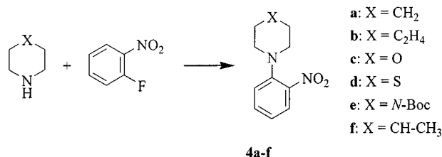
Scheme 1. Synthesis of nitroamines 4a-f
