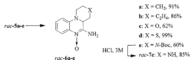
Scheme 4. Reductive cyclization of cyanoamines 5a–e
