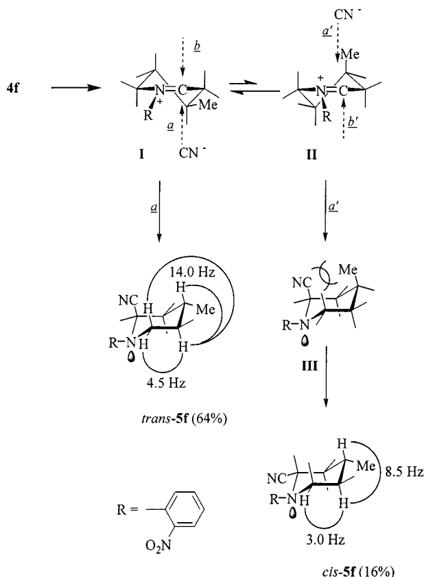
Scheme 3. Cyanide addition onto iminiums I and II
