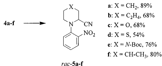
Scheme 2. Synthesis of cyanoamines 5a-f
