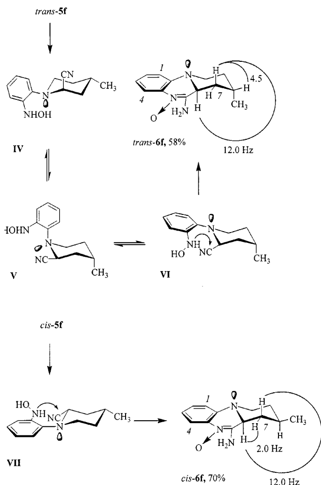
Scheme 5. Stereochemical pathway for the reductive ring-closure of trans - and cis - 5f
