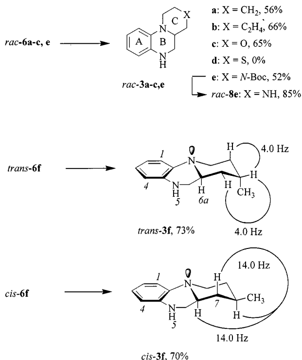
Scheme 6. Synthesis of the tetrahydroquinoxalines 3
